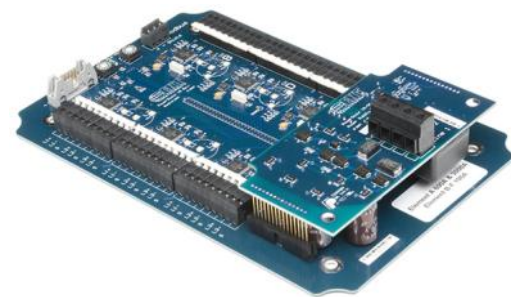
PowerScout™ 18 N version circuit board.
